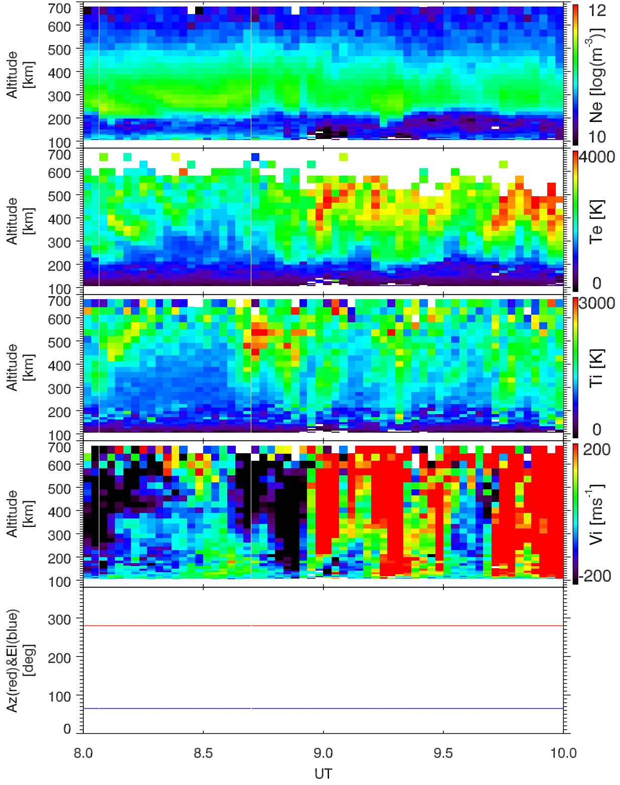
EISCAT 2003-11-28_08_10UT_tau0_120@32m.
