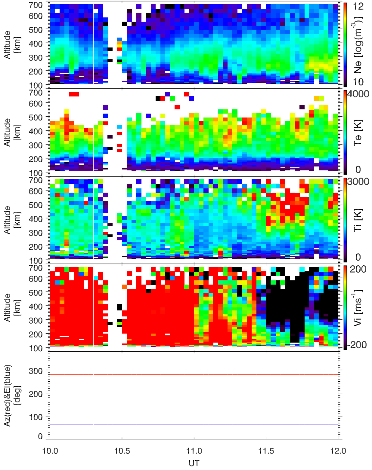
EISCAT 2003-11-28_10_12UT_tau0_120@32m.
