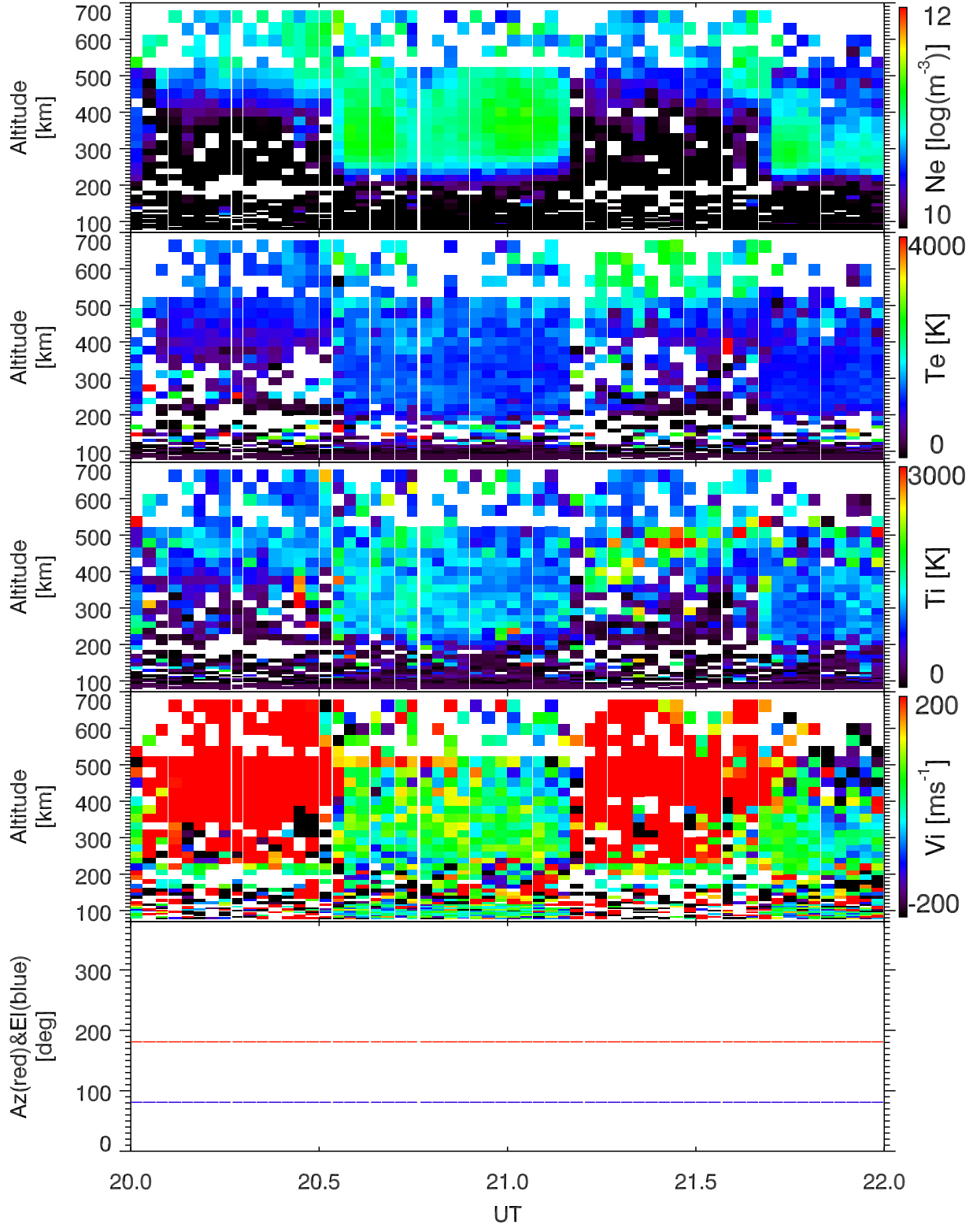
EISCAT 2004-02-18_20_22UT_steffe_120@42m.
