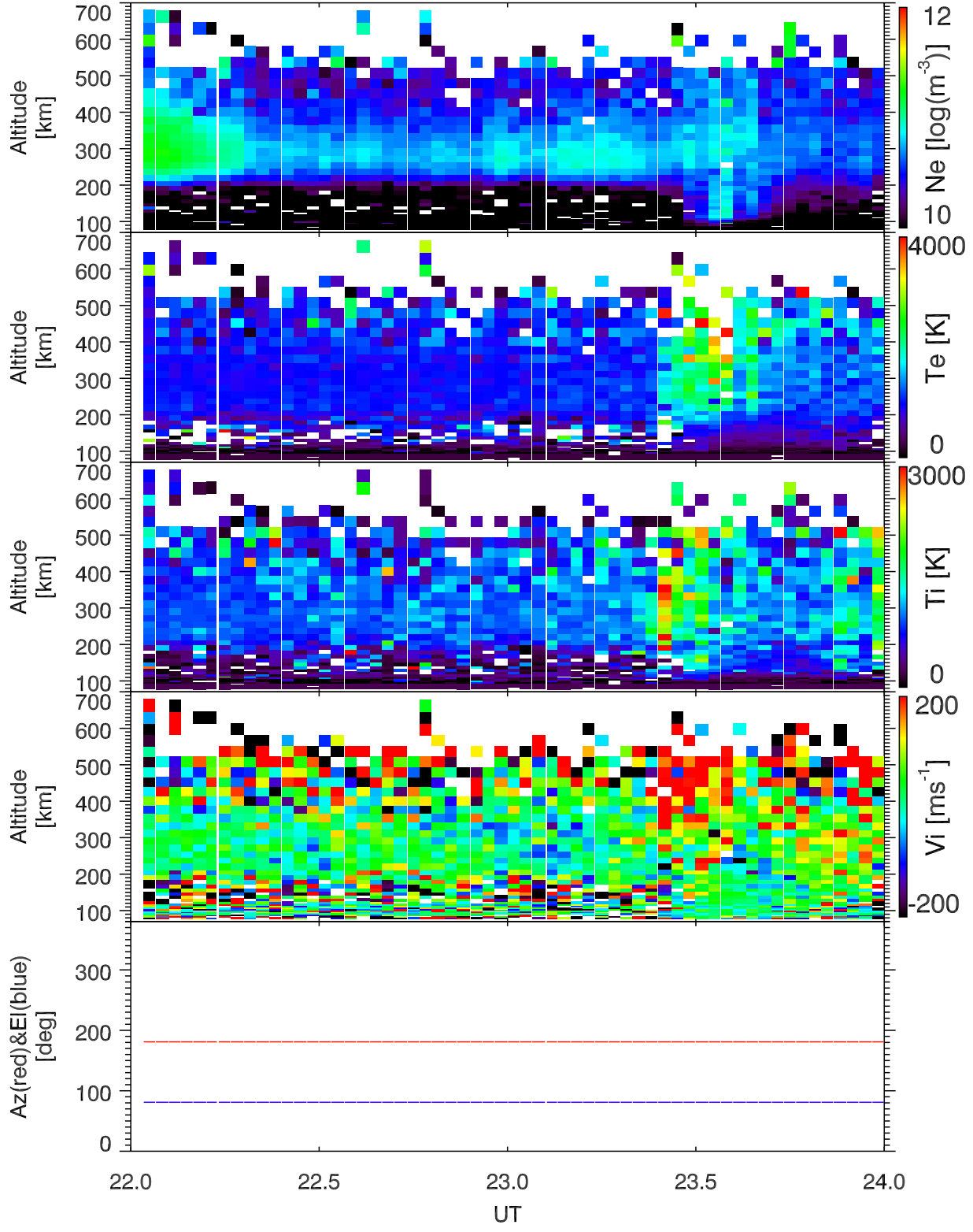
EISCAT 2004-02-19_22_24UT_steffe_120@42m.
