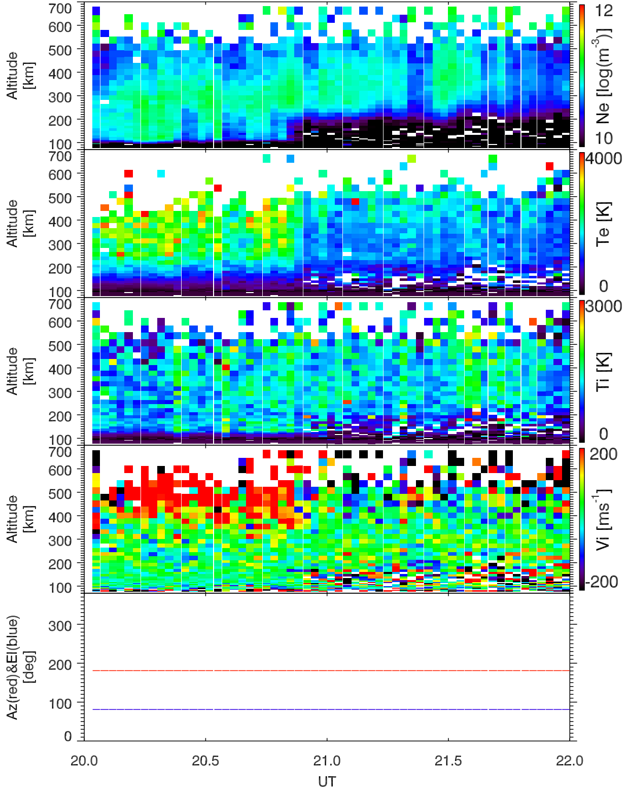
EISCAT 2004-02-21_20_22UT_steffe_120@42m.
