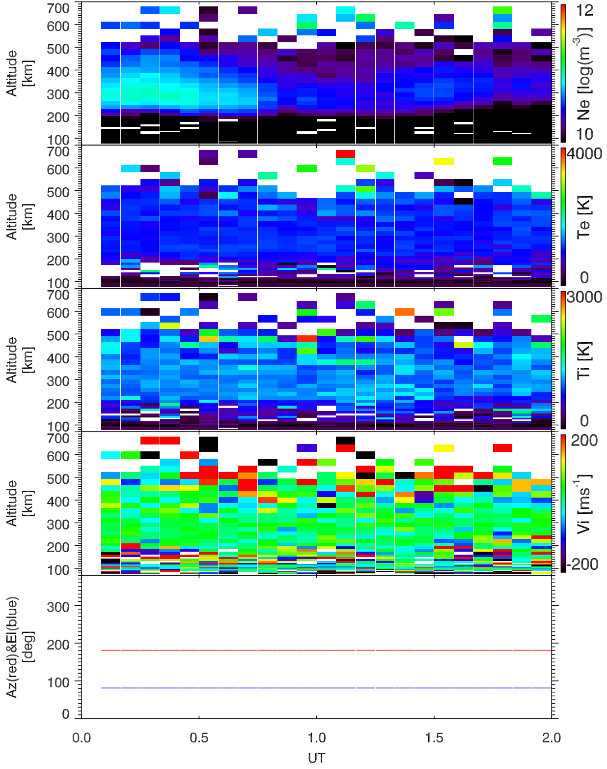
EISCAT 2004-02-22_00_02UT_steffe_120@42m.
