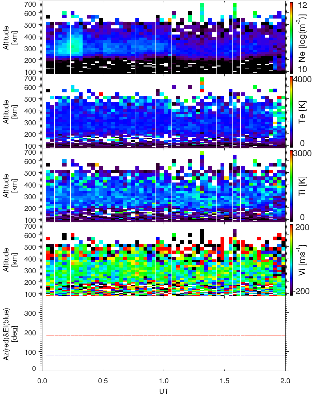
EISCAT 2004-02-24_00_02UT_steffe_120@42m.
