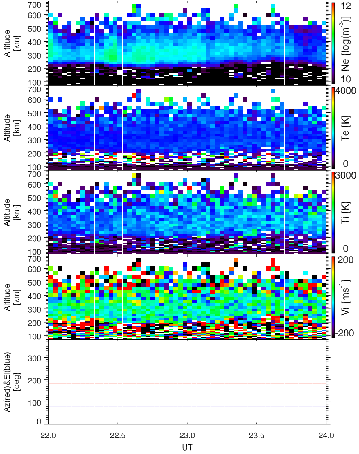
EISCAT 2004-02-24_22_24UT_steffe_120@42m.
