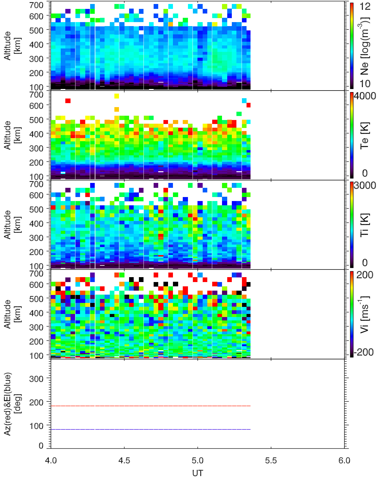
EISCAT 2004-03-30_04_06UT_steffe_120@42m.
