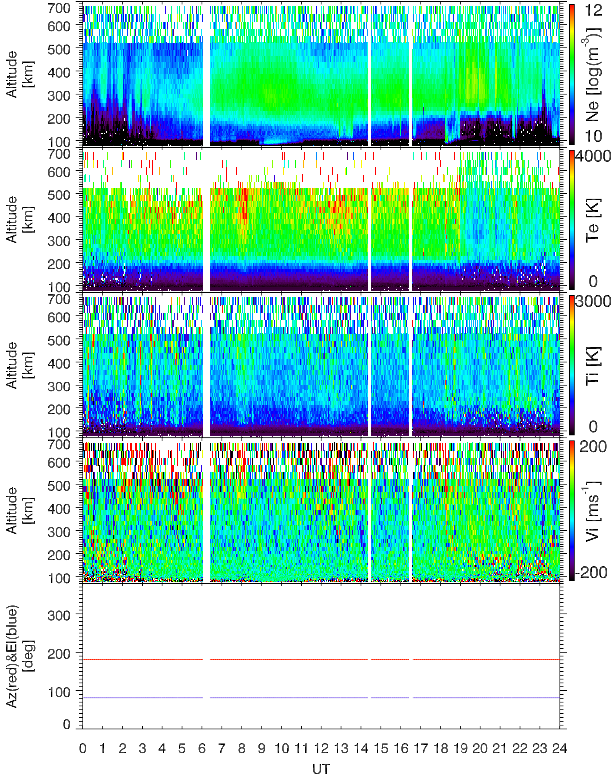
EISCAT 2004-03-31_00_24UT_steffe_120@42m.
