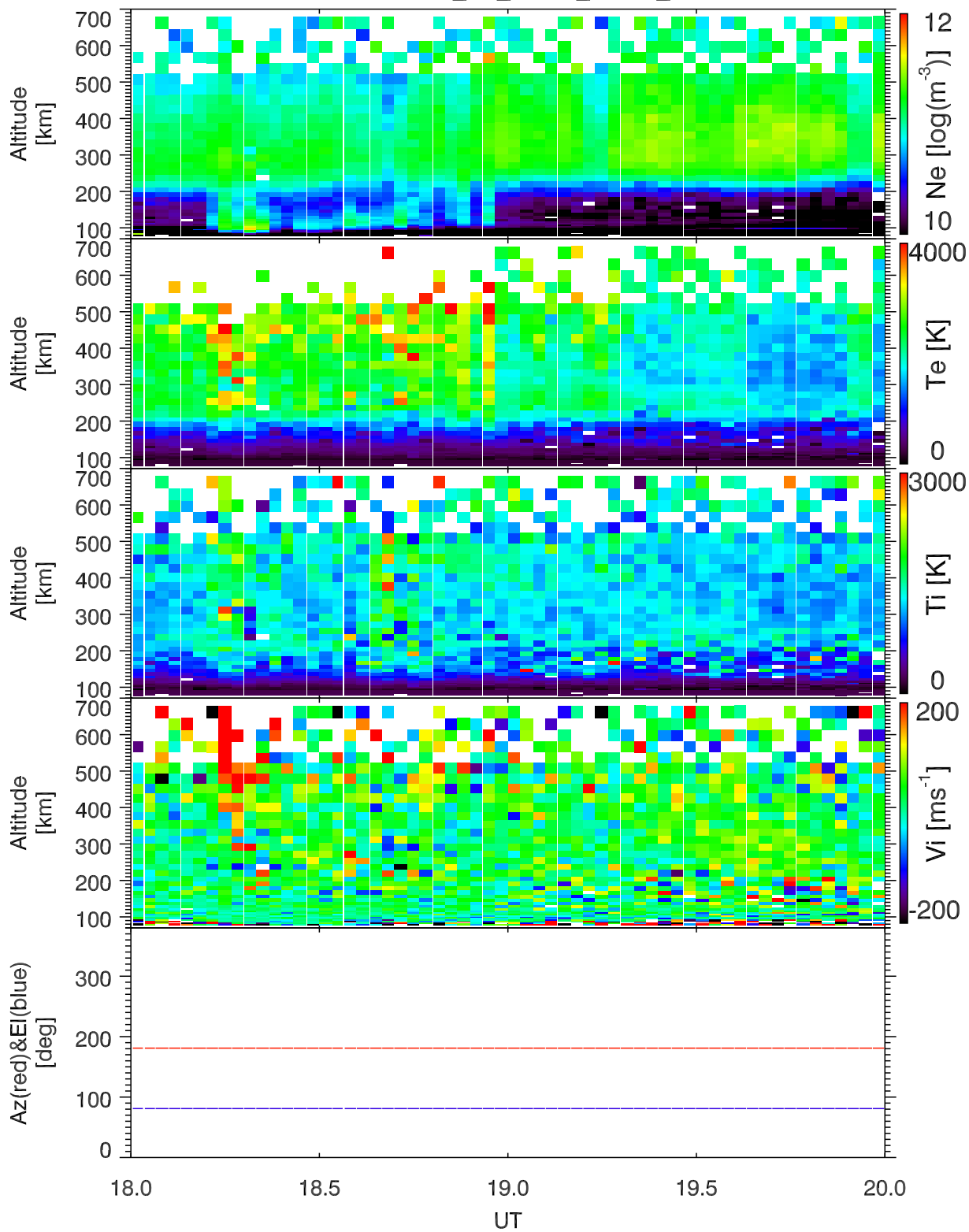
EISCAT 2004-03-31_18_20UT_steffe_120@42m.
