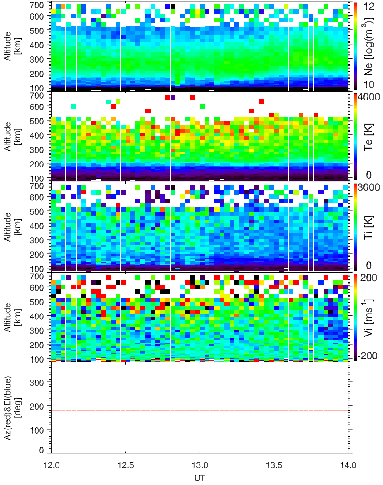
EISCAT 2004-04-01_12_14UT_steffe_120@42m.
