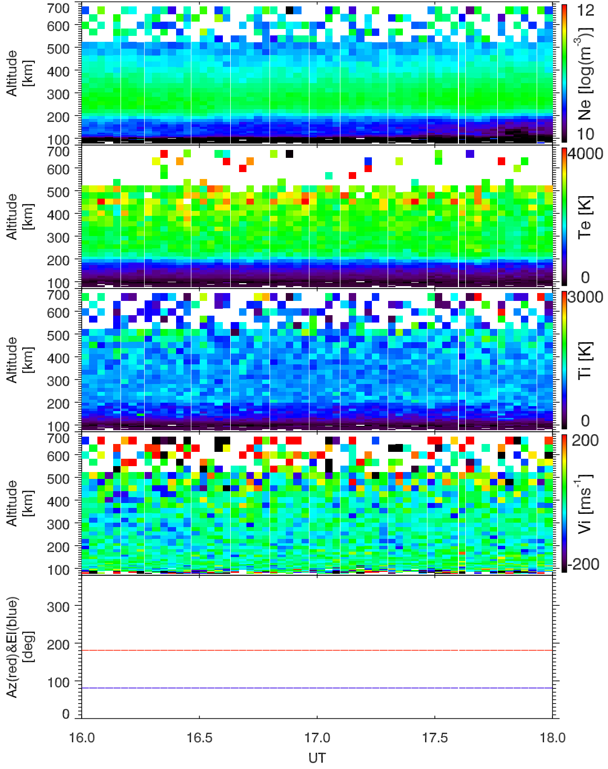
EISCAT 2004-04-01_16_18UT_steffe_120@42m.
