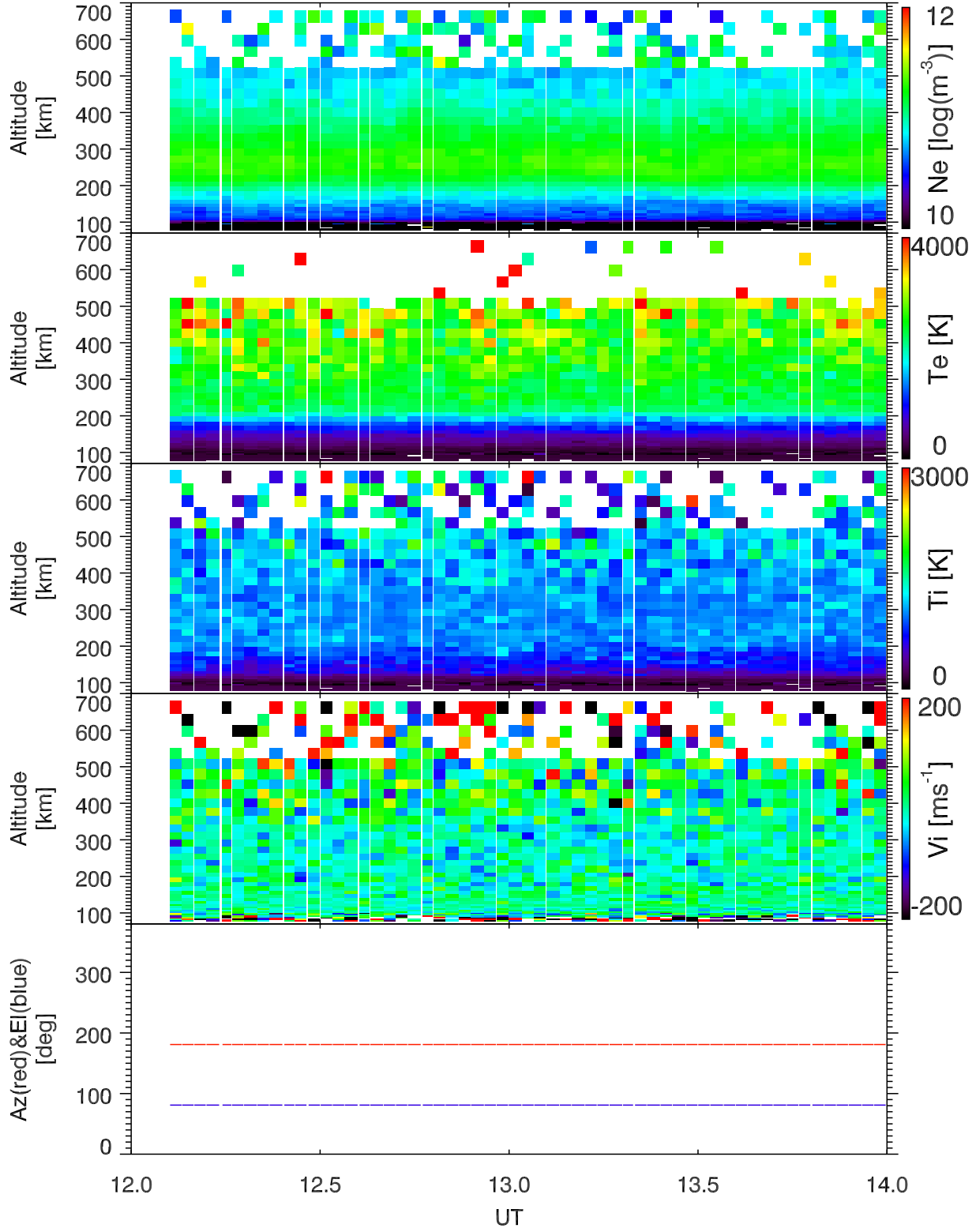
EISCAT 2004-04-02_12_14UT_steffe_120@42m.
