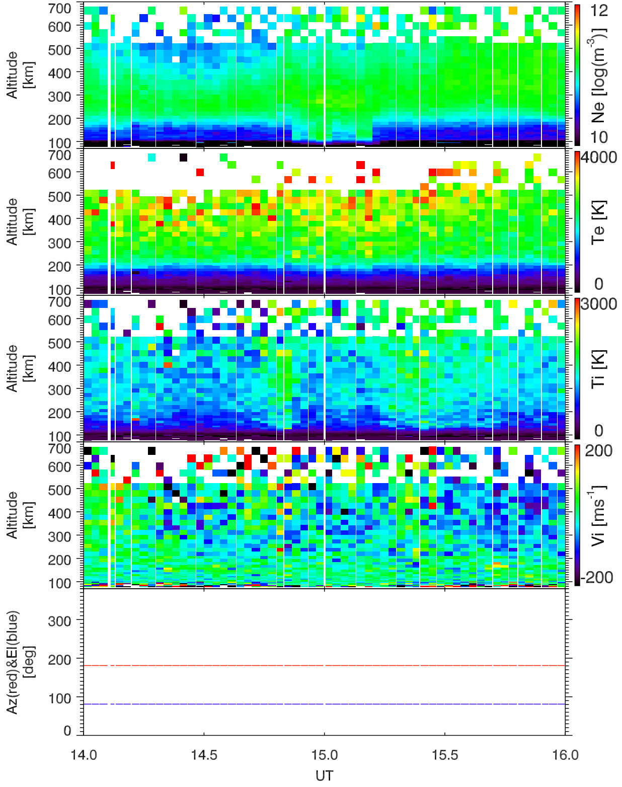
EISCAT 2004-04-03_14_16UT_steffe_120@42m.
