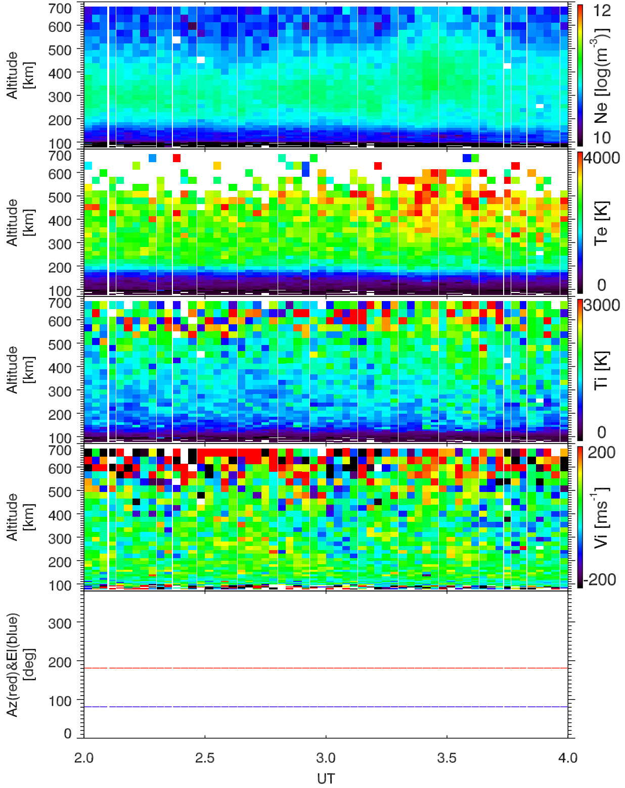
EISCAT 2004-05-25_02_04UT_steffe_120@42m.
