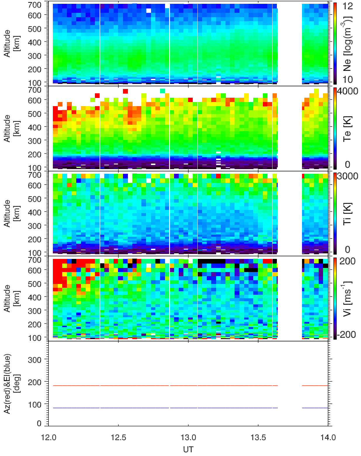
EISCAT 2004-06-01_12_14UT_tau0_120@42m.
