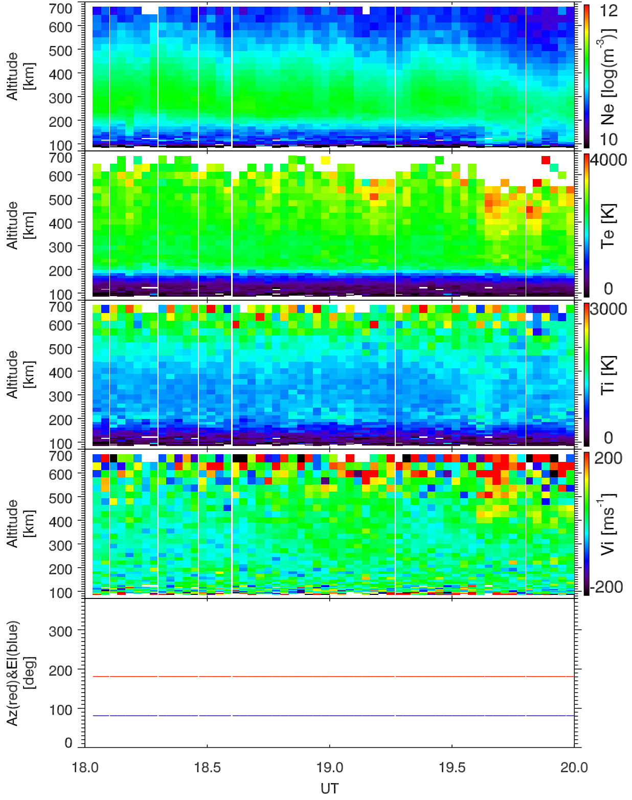
EISCAT 2004-06-01_18_20UT_tau0_120@42m.
