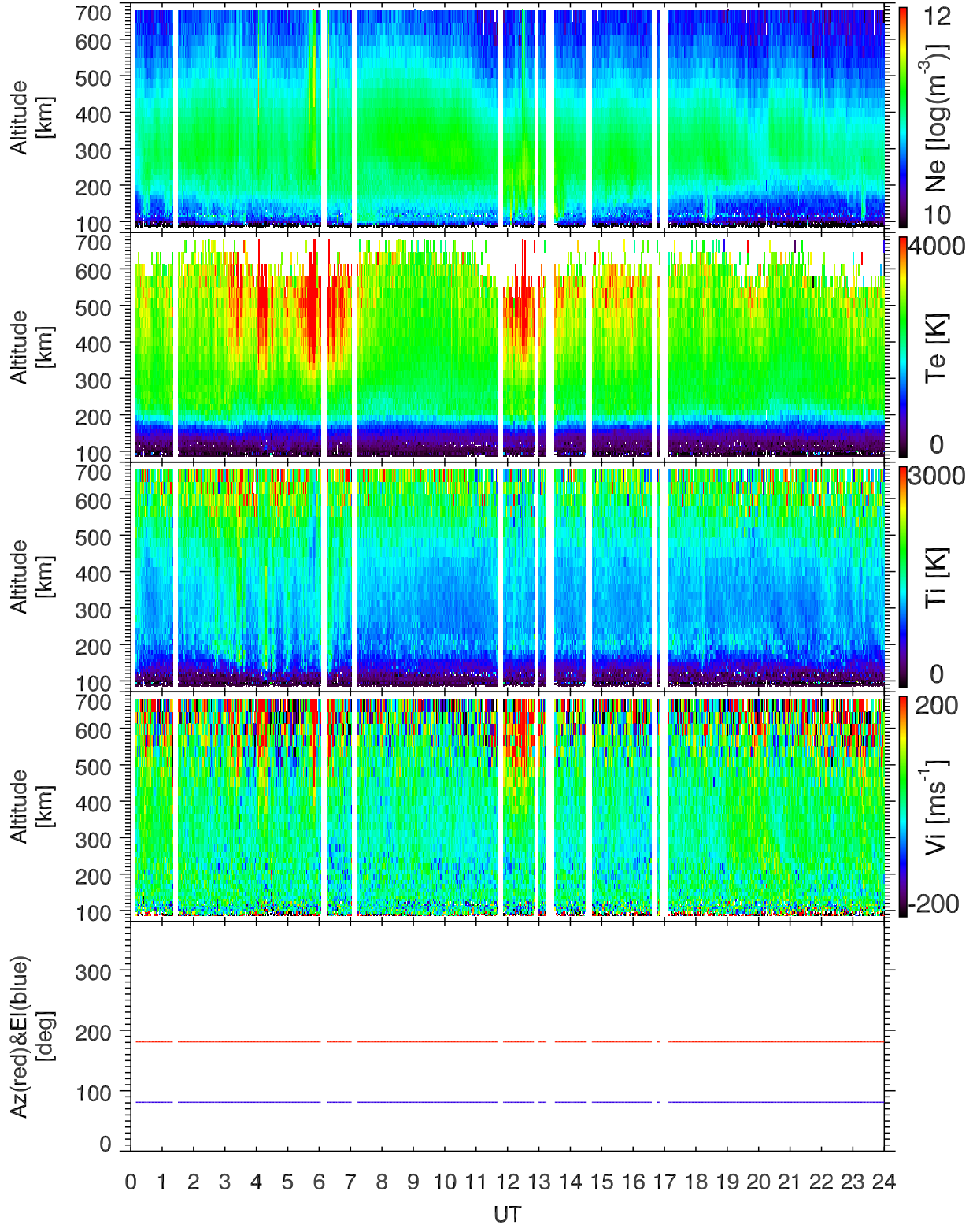
EISCAT 2004-06-02_00_24UT_tau0_120@42m.
