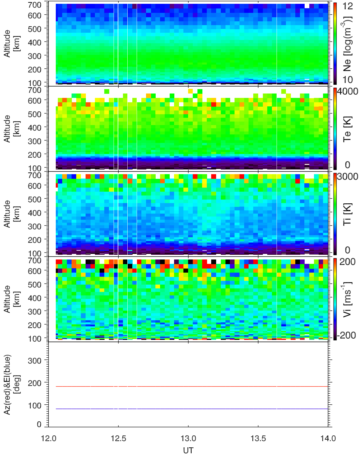
EISCAT 2004-06-03_12_14UT_tau0_120@42m.
