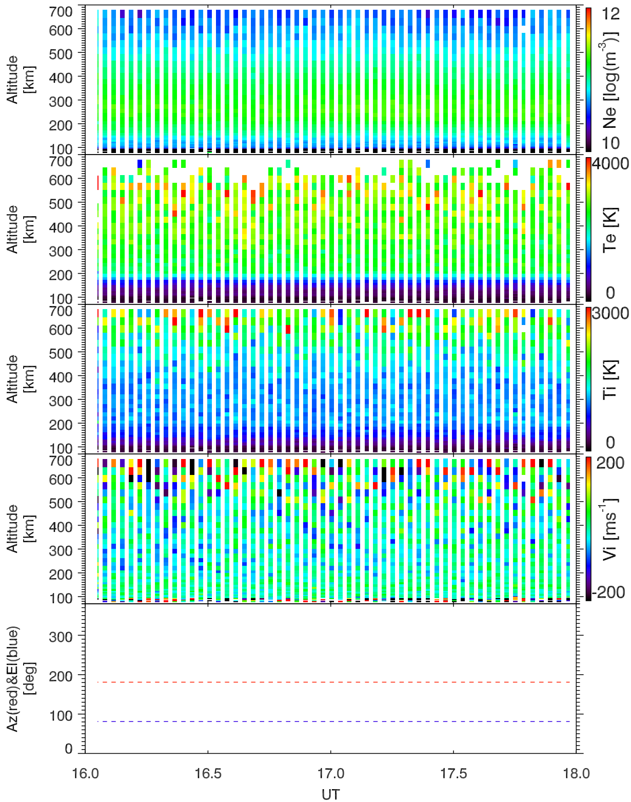
EISCAT 2004-06-04_16_18UT_all_all@42m.
