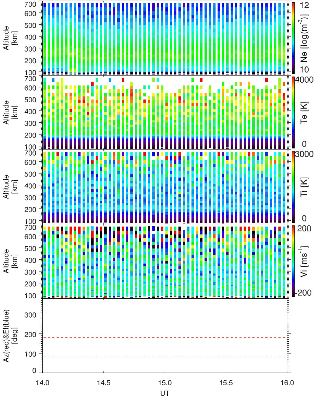
EISCAT 2004-06-06_14_16UT_steffe_ant@42m.
