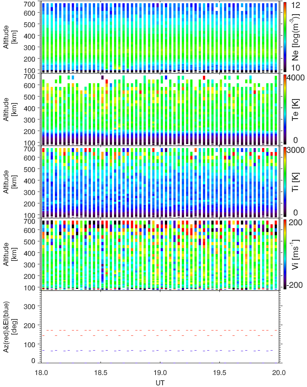
EISCAT 2004-06-11_18_20UT_steffe_ant@32m.
