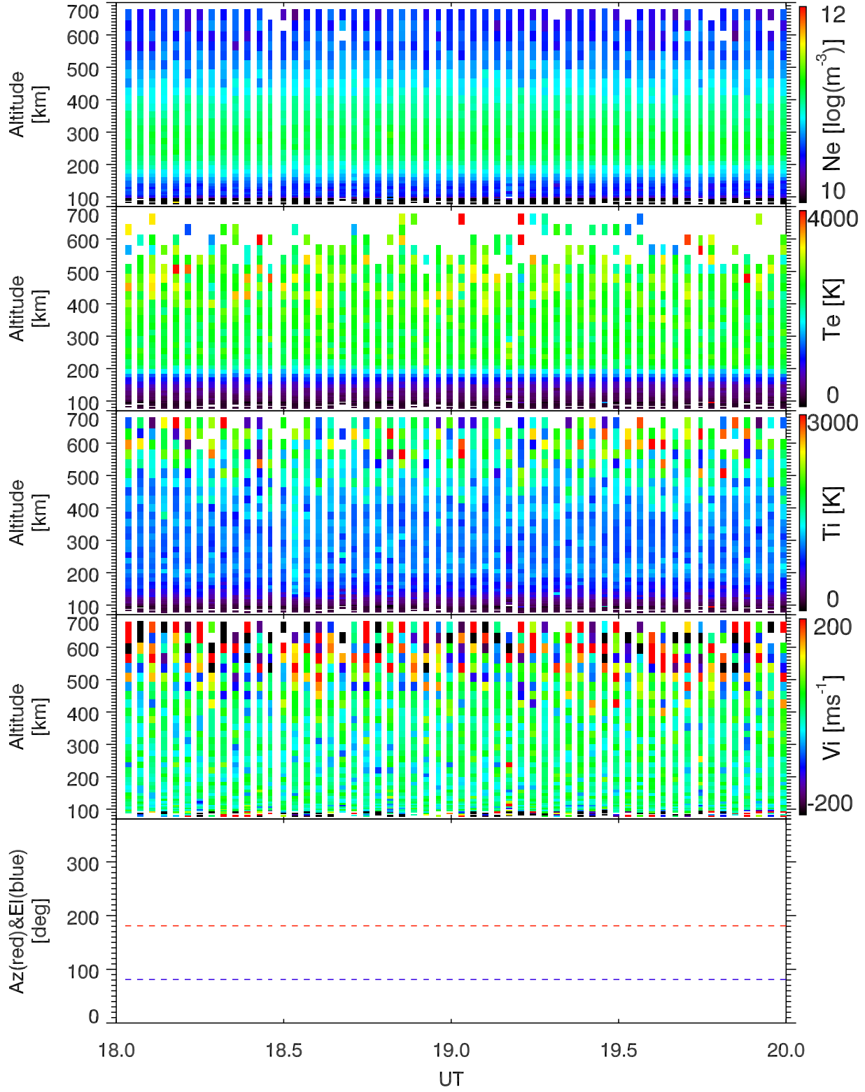
EISCAT 2004-06-11_18_20UT_steffe_ant@42m.
