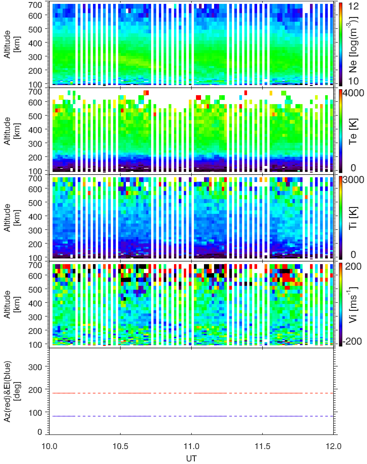
EISCAT 2005-04-19_10_12UT_tau0_all@42m.
