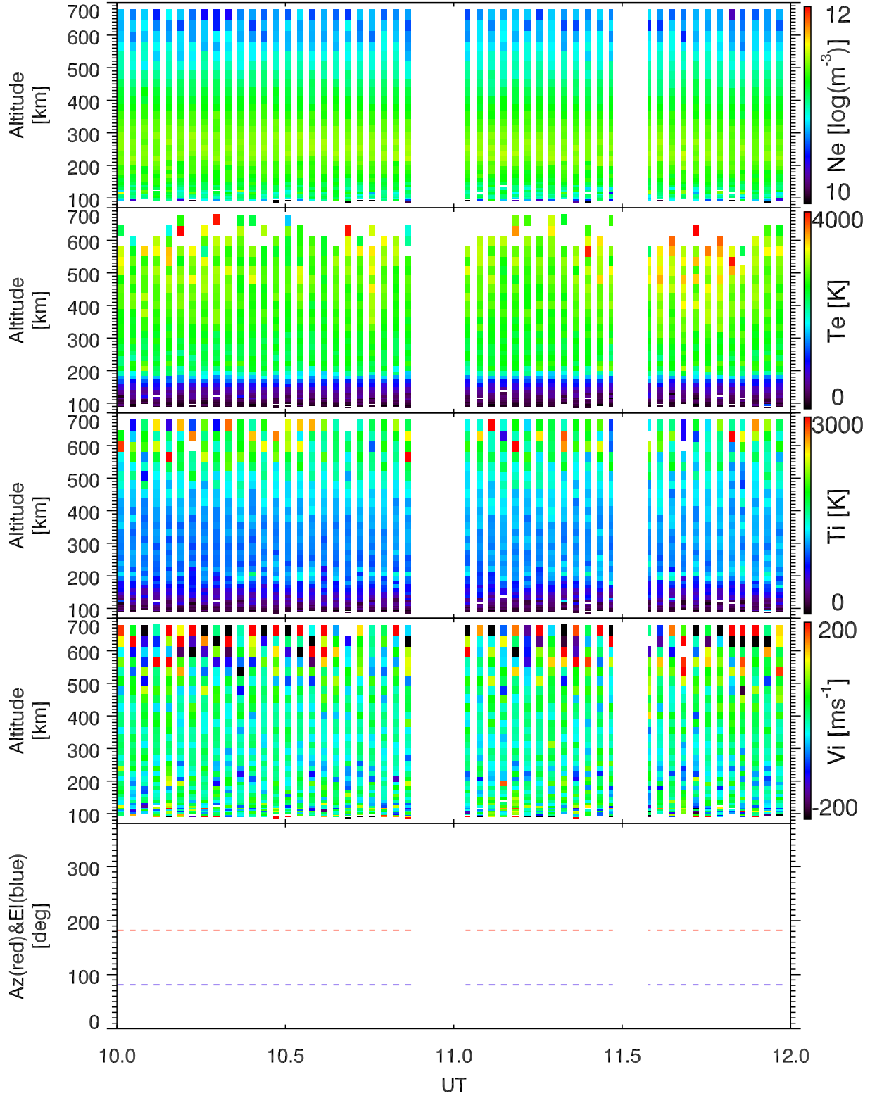
EISCAT 2005-07-01_10_12UT_tau0_ant@42m.
