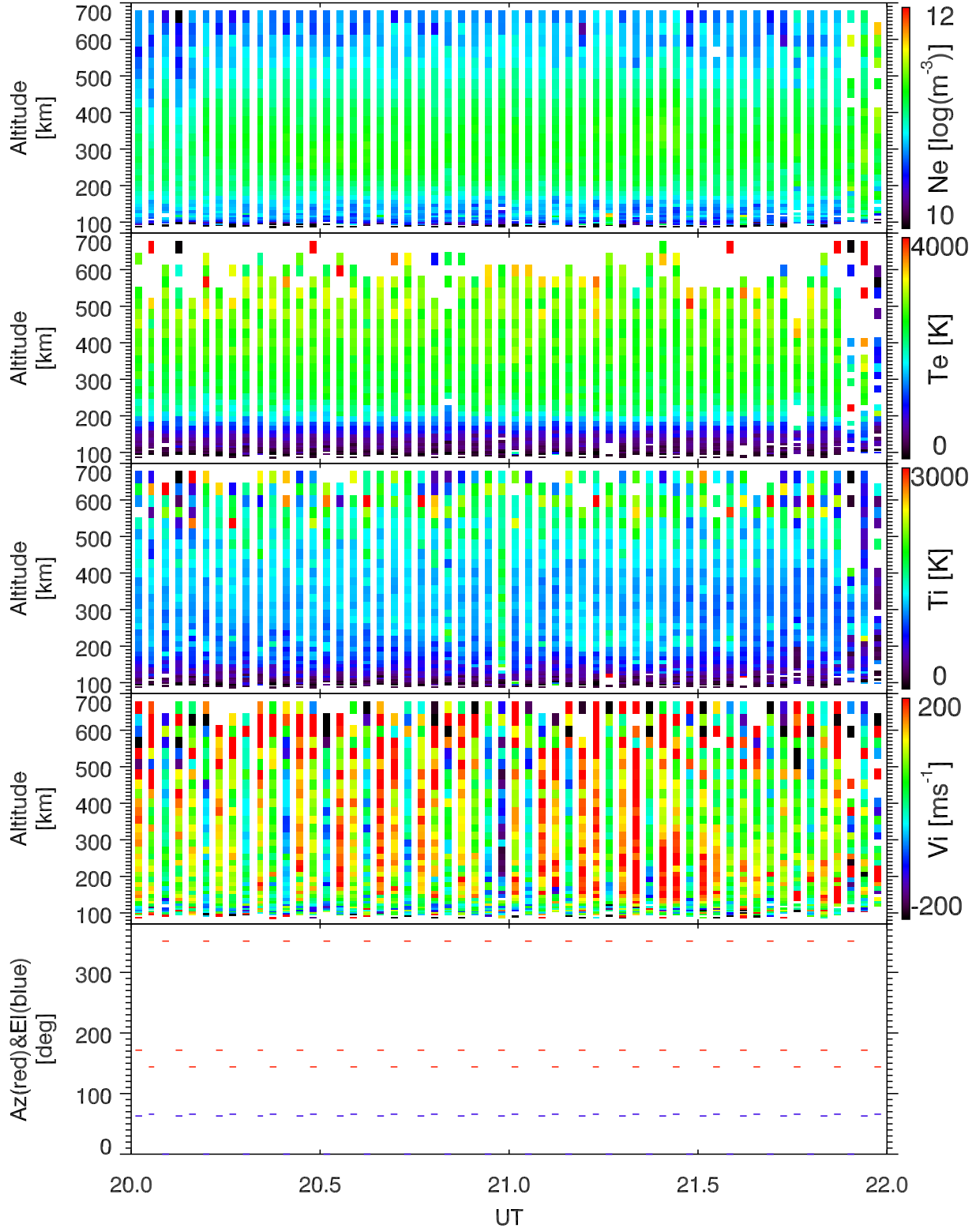
EISCAT 2005-07-01_20_22UT_tau0_ant@32m.
