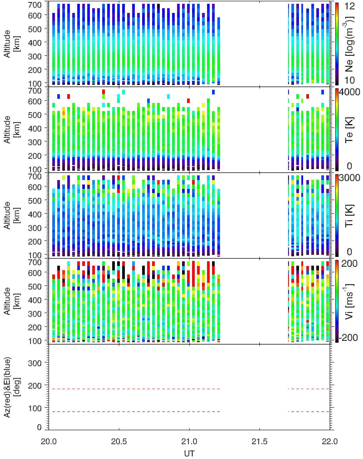
EISCAT 2005-07-22_20_22UT_tau0_ant@42m.
