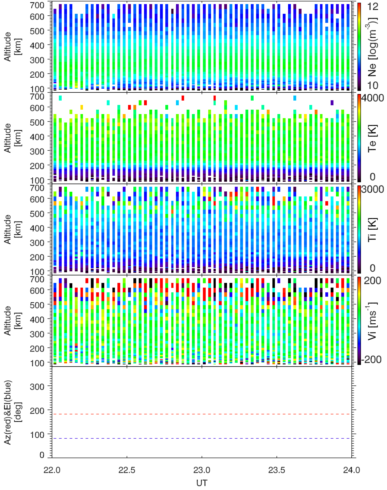
EISCAT 2005-07-22_22_24UT_tau0_ant@42m.
