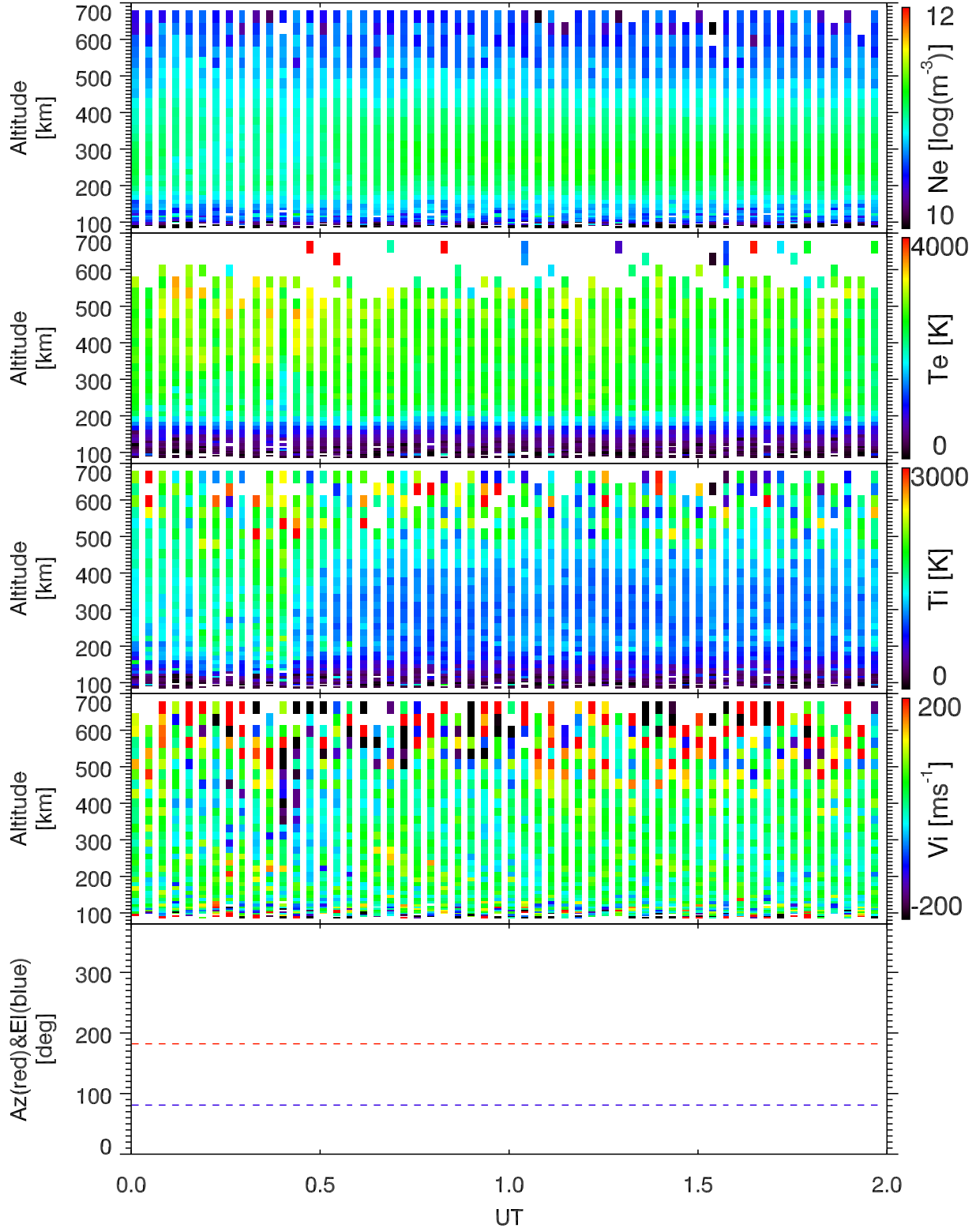
EISCAT 2005-07-23_00_02UT_tau0_ant@42m.
