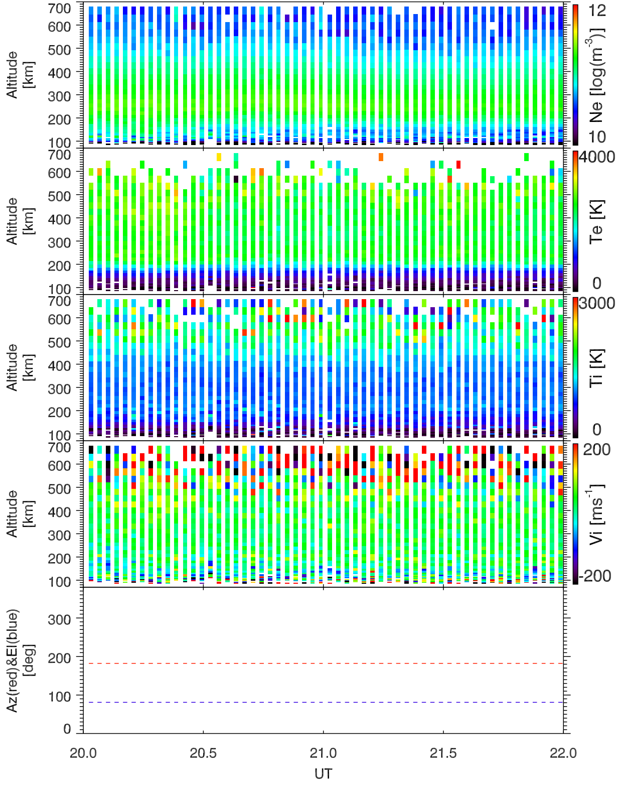
EISCAT 2005-07-23_20_22UT_tau0_ant@42m.
