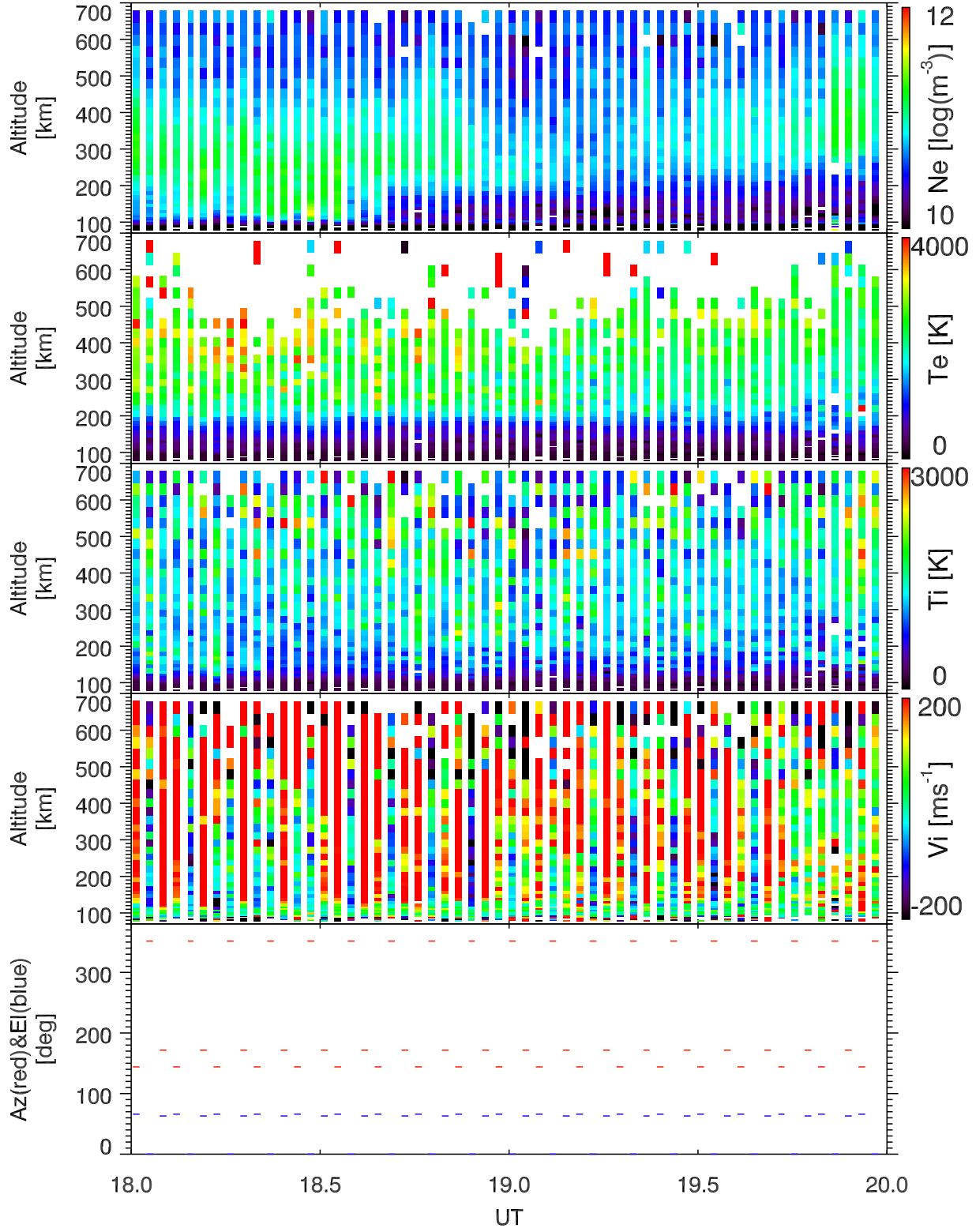
EISCAT 2005-09-02_18_20UT_steffe_ant@32m.
