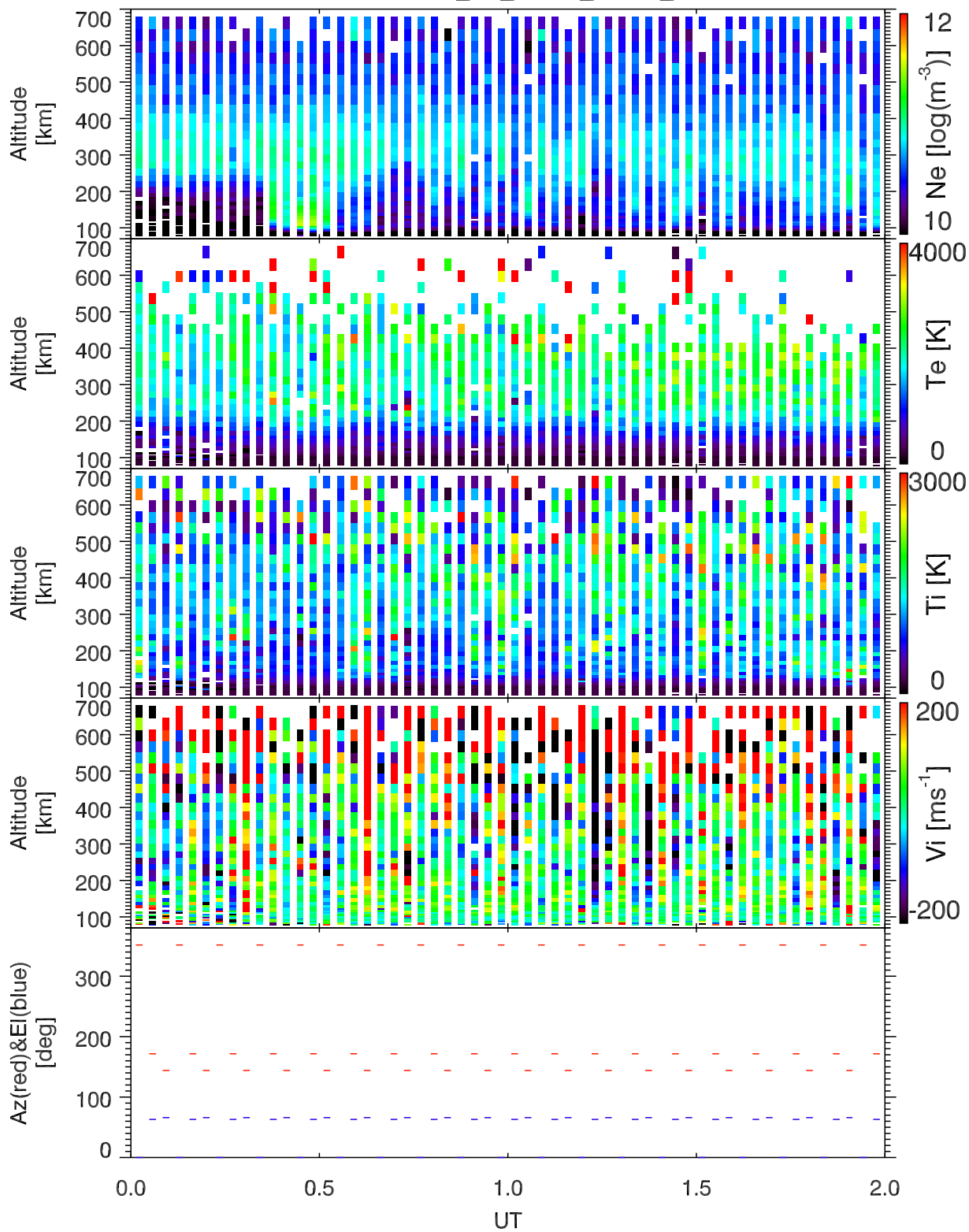
EISCAT 2005-09-04_00_02UT_steffe_ant@32m.
