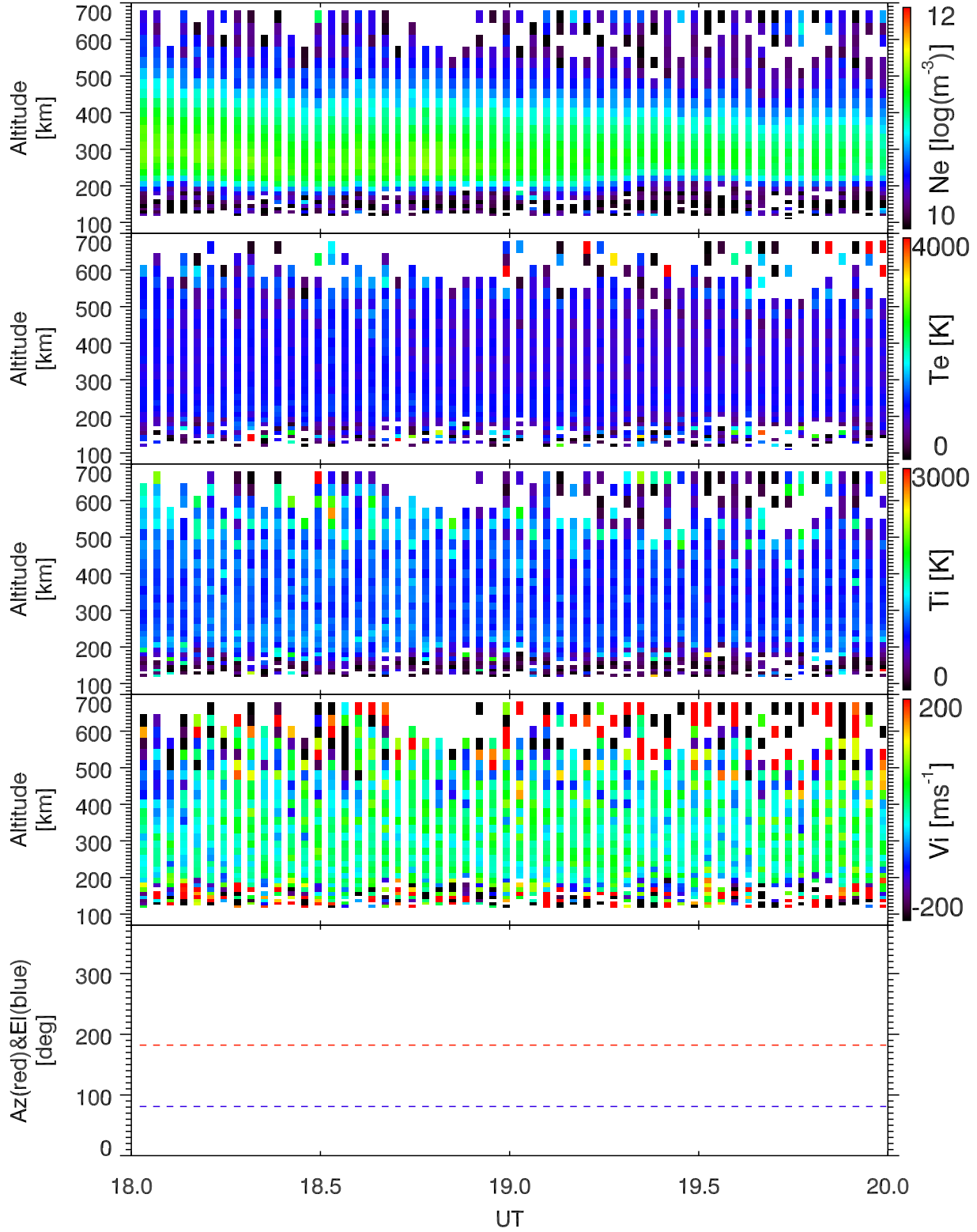
EISCAT 2005-11-08_18_20UT_tau0_ant@42m.
