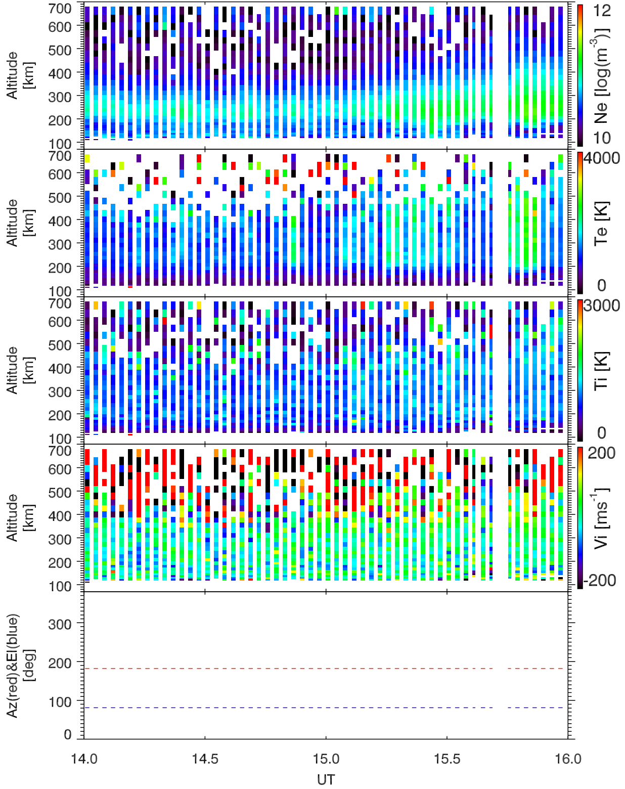
EISCAT 2005-11-09_14_16UT_tau0_ant@42m.
