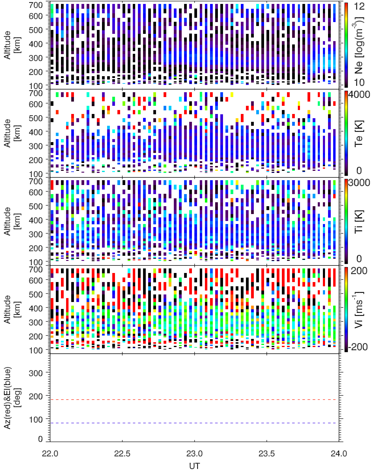
EISCAT 2005-11-09_22_24UT_tau0_ant@42m.
