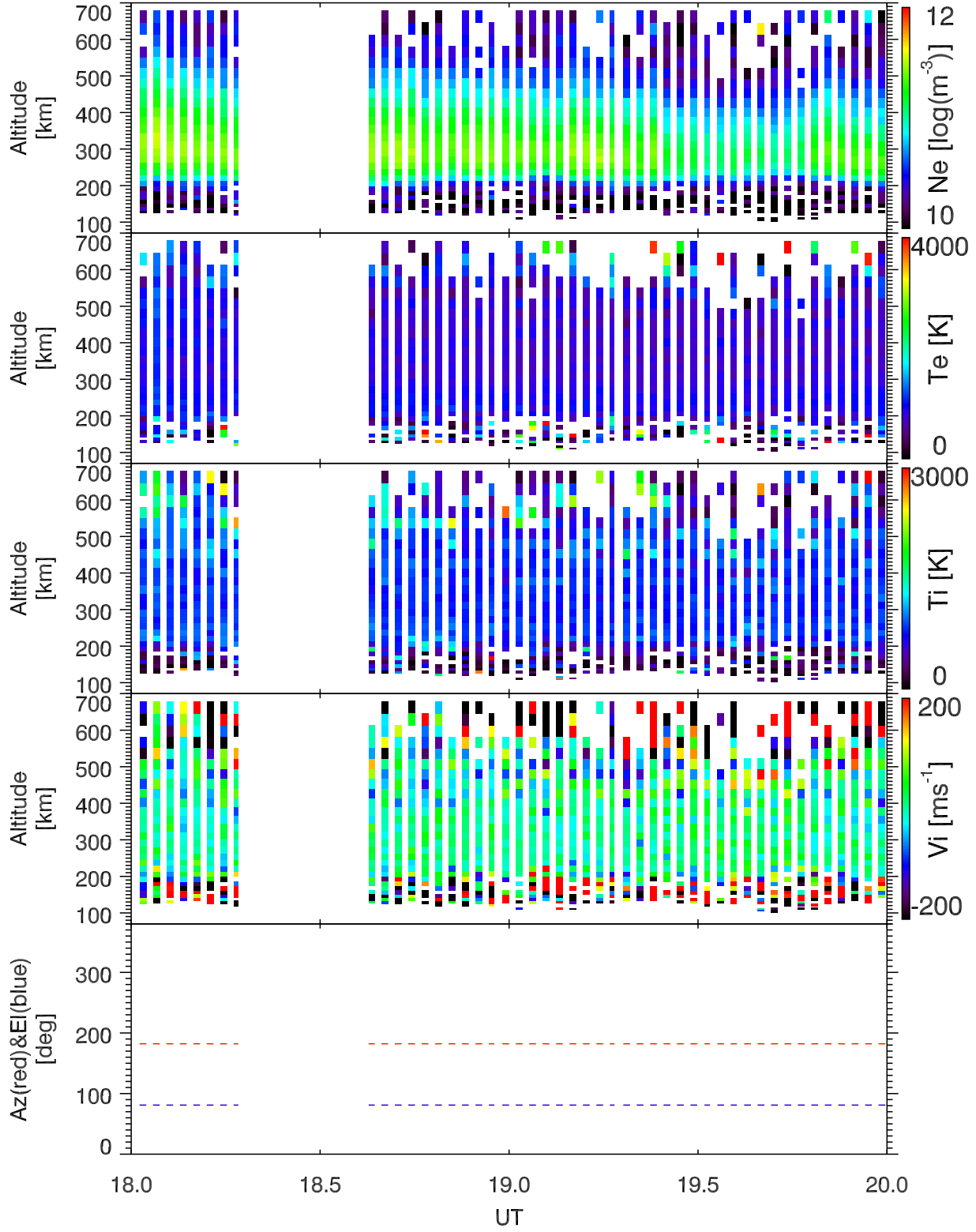
EISCAT 2005-11-10_18_20UT_tau0_ant@42m.
