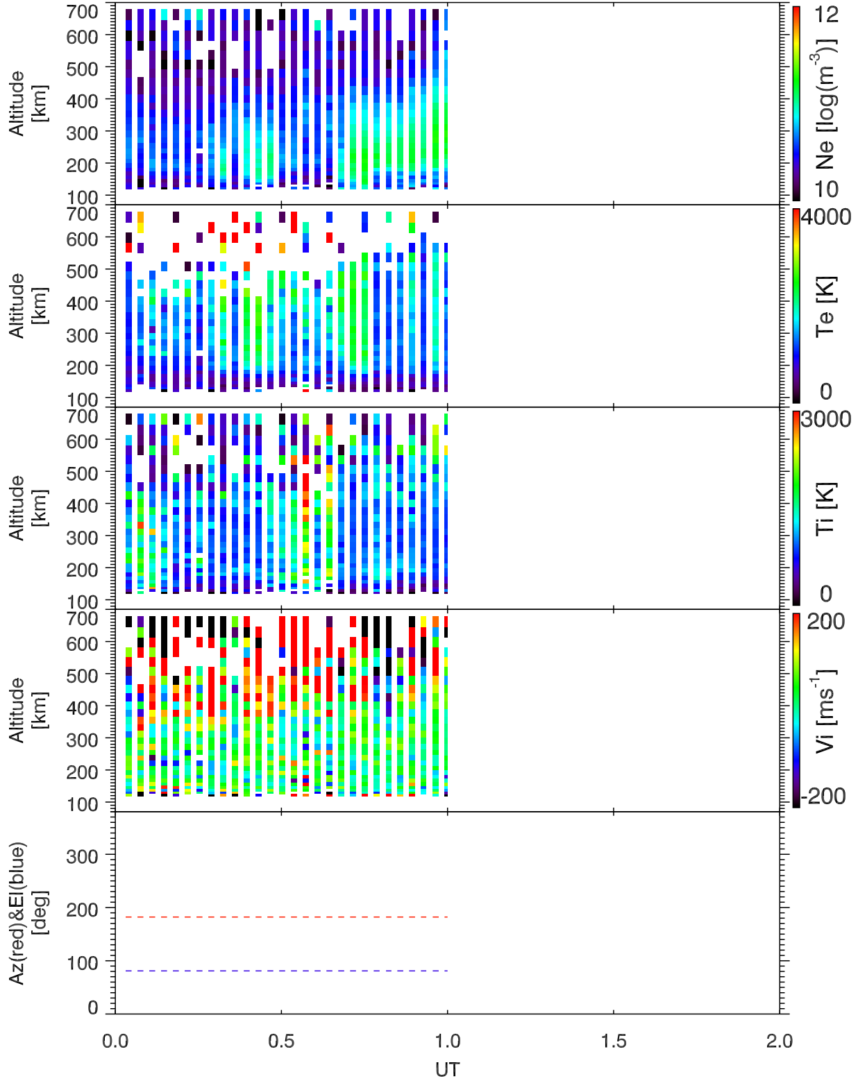
EISCAT 2005-11-11_00_02UT_tau0_ant@42m.
