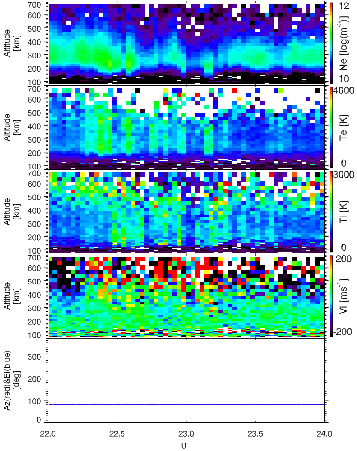
EISCAT 2006-02-05_22_24UT_steffe_120@42m.
