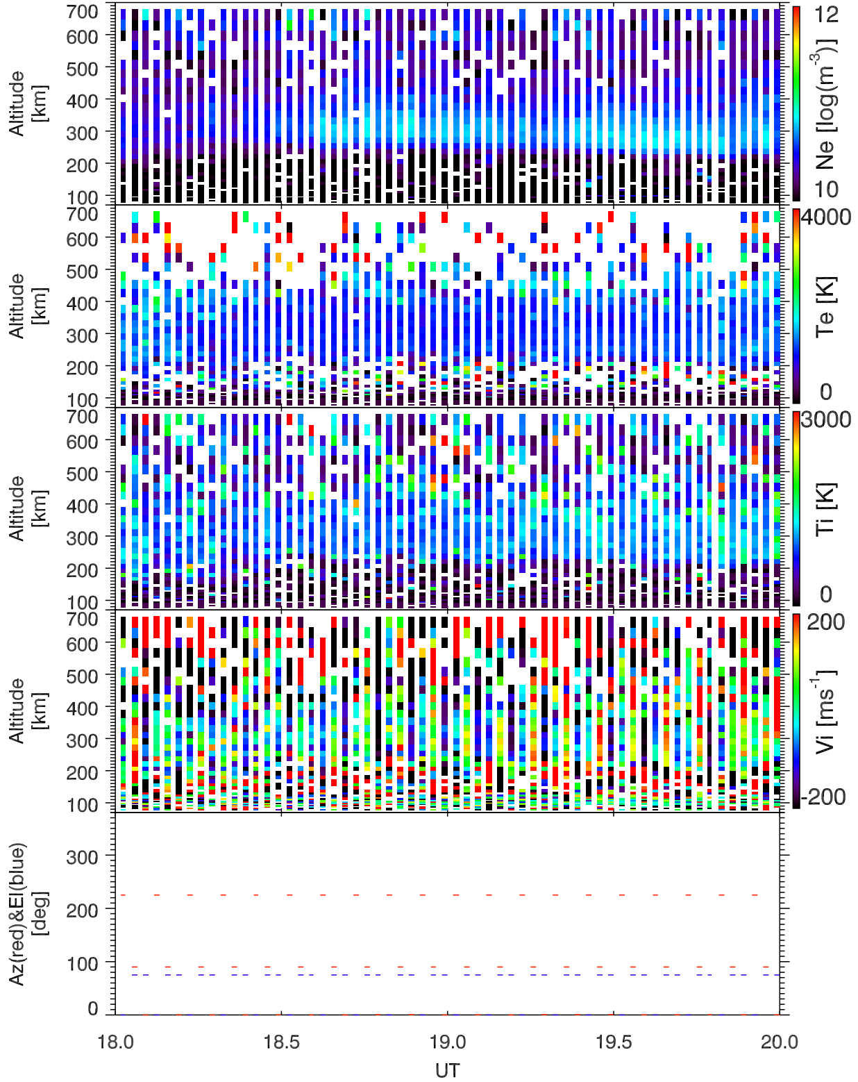
EISCAT 2006-02-20_18_20UT_steffe_ant@32m.
