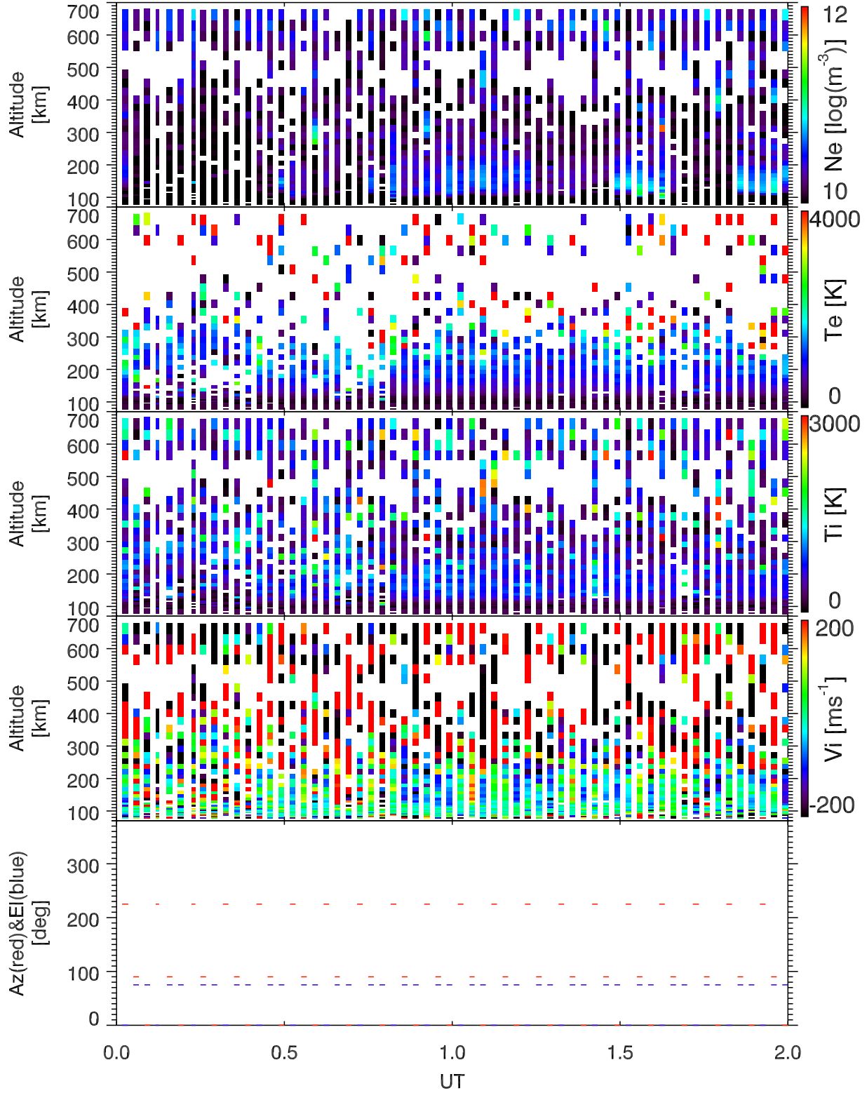
EISCAT 2006-02-21_00_02UT_steffe_ant@32m.
