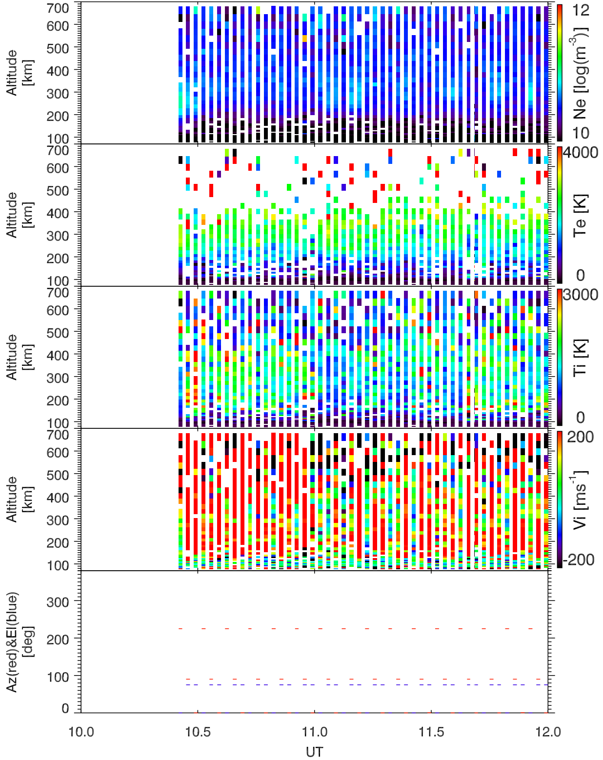
EISCAT 2006-02-21_10_12UT_steffe_ant@32m.
