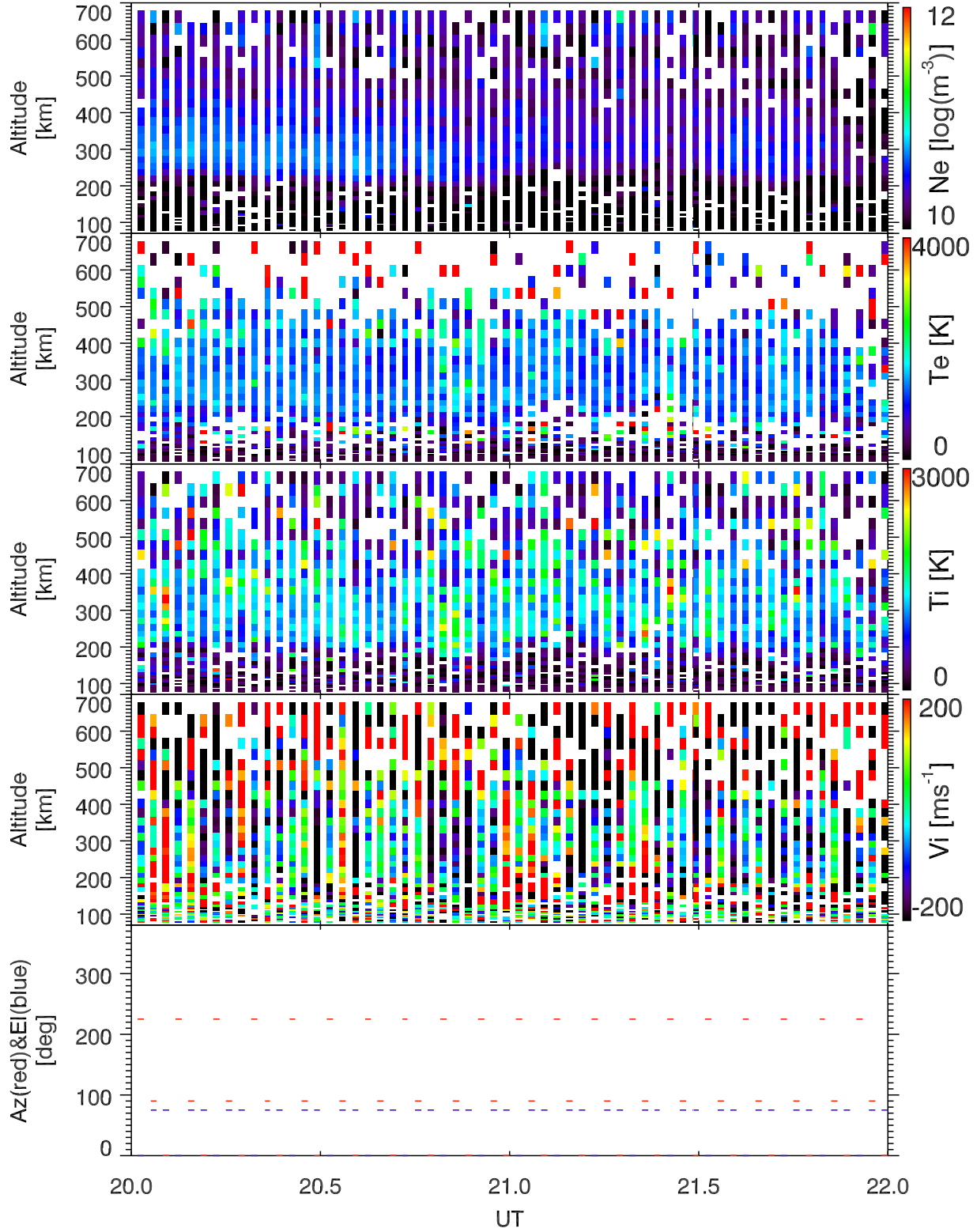
EISCAT 2006-02-21_20_22UT_steffe_ant@32m.
