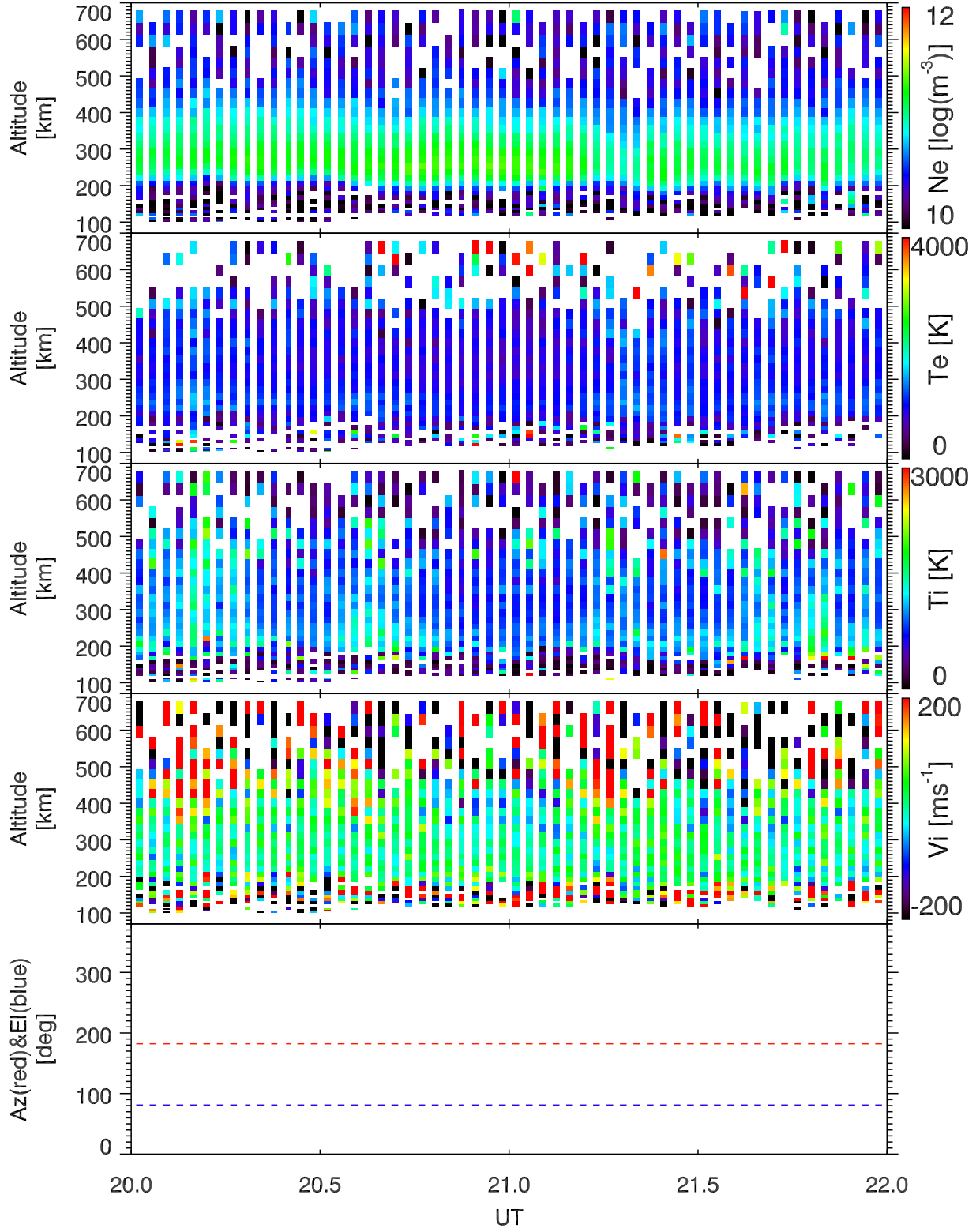
EISCAT 2006-09-22_20_22UT_tau0_ant@42m.
