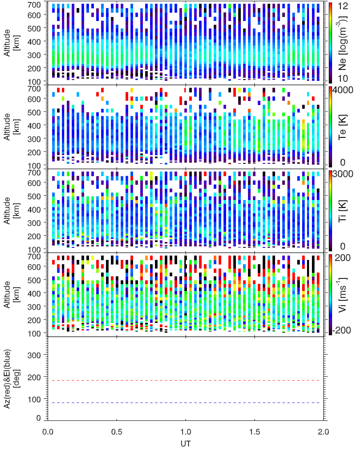
EISCAT 2006-09-23_00_02UT_tau0_ant@42m.
