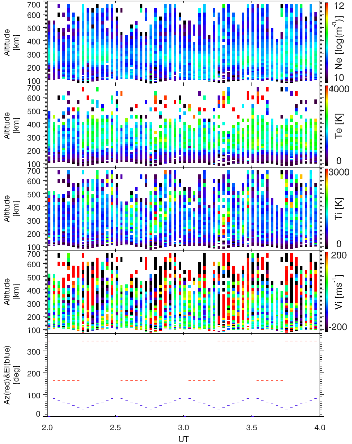
EISCAT 2006-09-23_02_04UT_tau0_ant@32m.
