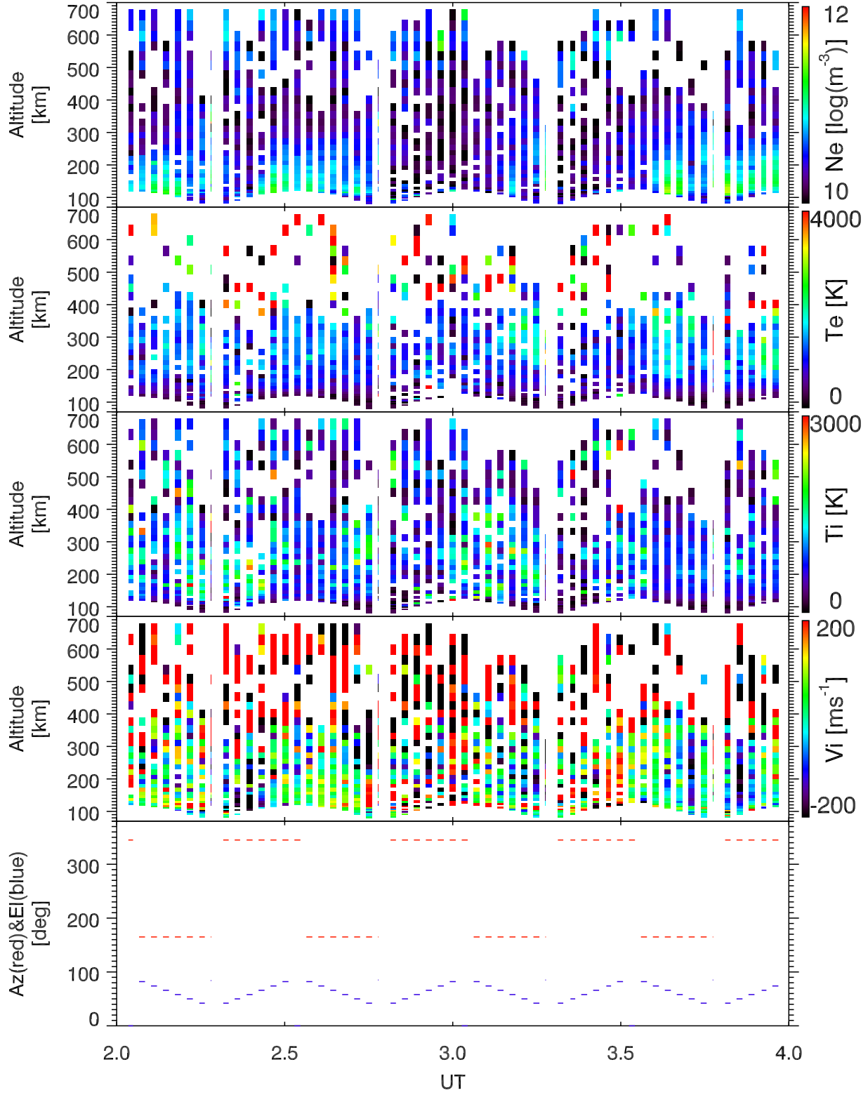
EISCAT 2006-12-14_02_04UT_tau0_ant@32m.
