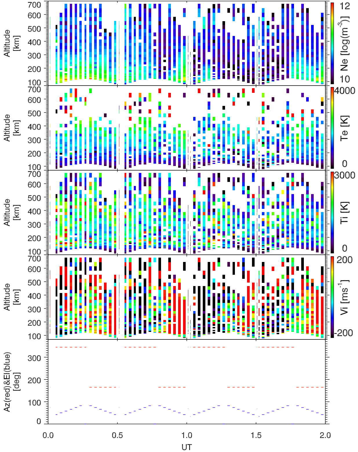
EISCAT 2006-12-15_00_02UT_tau0_ant@32m.
