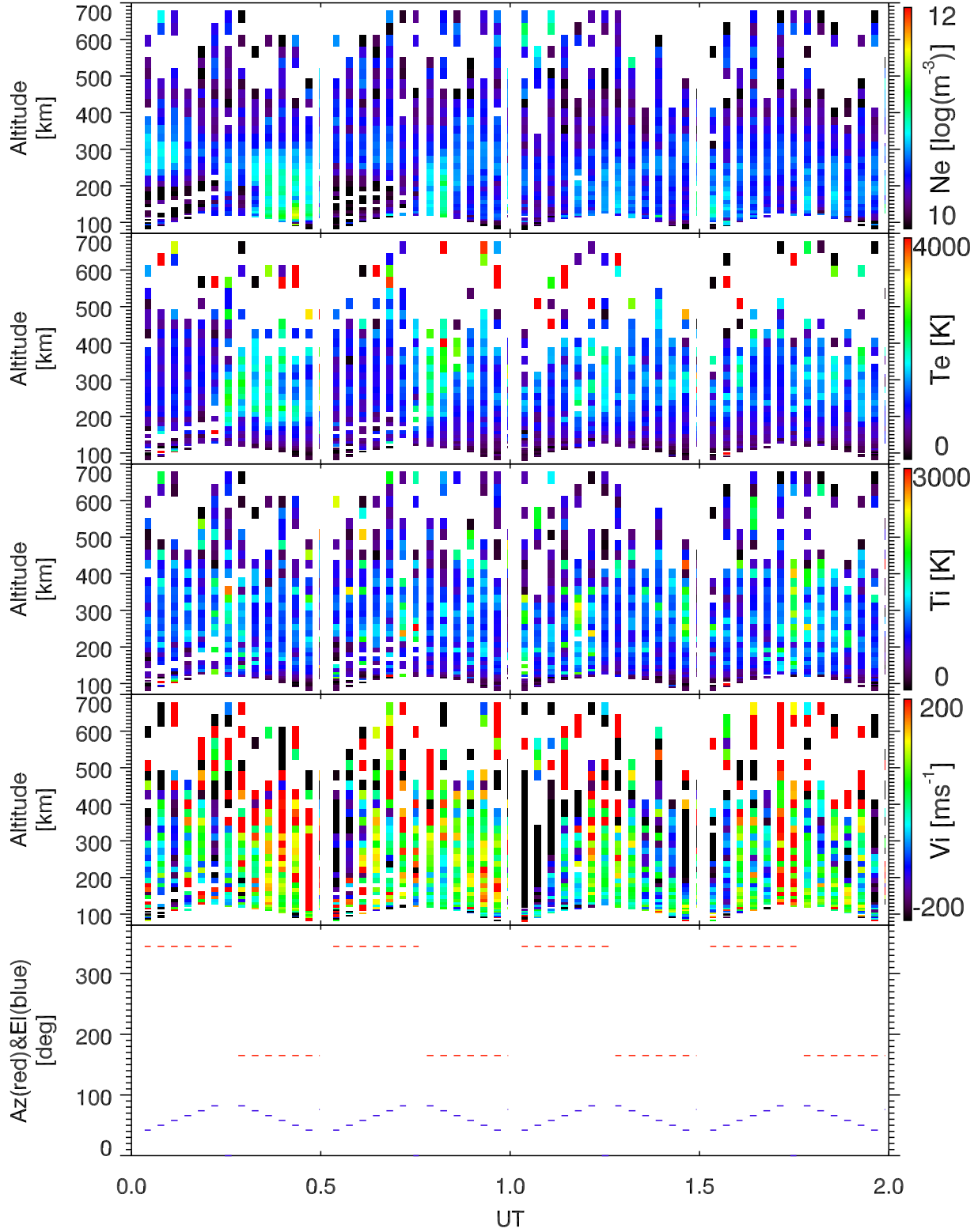
EISCAT 2006-12-19_00_02UT_tau0_ant@32m.
