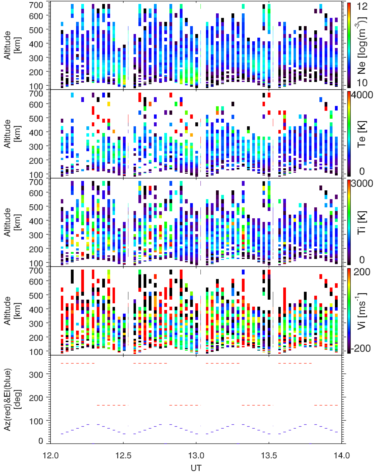
EISCAT 2006-12-21_12_14UT_tau0_ant@32m.
